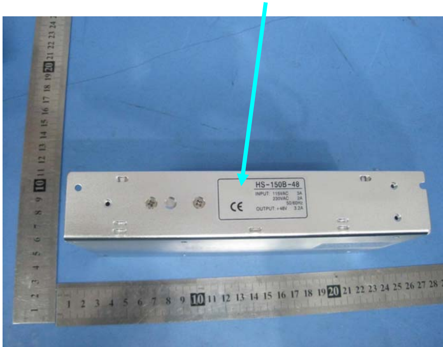
Proposed Label Location on EUT EUT Front View/proposed CE Mark Location
